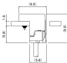
PA Receptacle (Standard type) + PA bottom type header (Extended length type)
